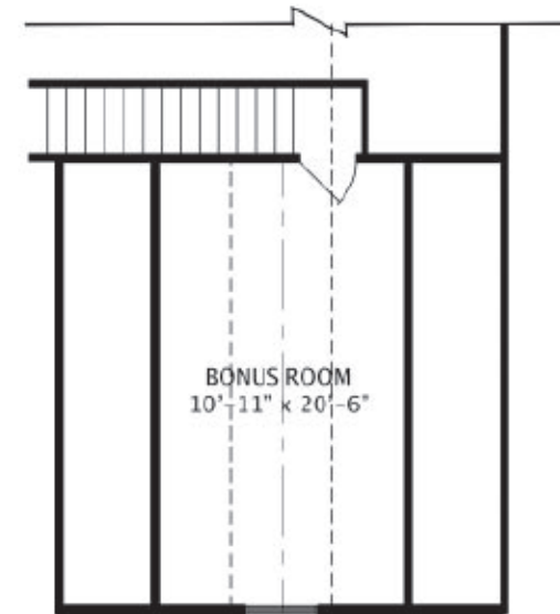
Optional Second Floor Plan
